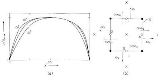
Figure 8. (a) Horizontal velocity u' at the upper surface of model convection cells for various values of R_B/R_C (as labelled) expressed as a ratio of their respective maximum values u'_{\max} (b) A small portion of the finite-difference grid indicating the volume element bounded by the surface S . Grid points are indicated by circles and \times 's. The four faces of S are individually labelled as 1, 2, 3 and 4. Conductive fluxes across each face are computed in terms of temperature at the grid points labelled \times . Advective fluxes are computed in terms of temperature at the points labelled with open circles and streamfunction at the points labelled with solid circles. COND_i is the conducted flux across the i th face; AD_i is the advected flux across the i th face.
