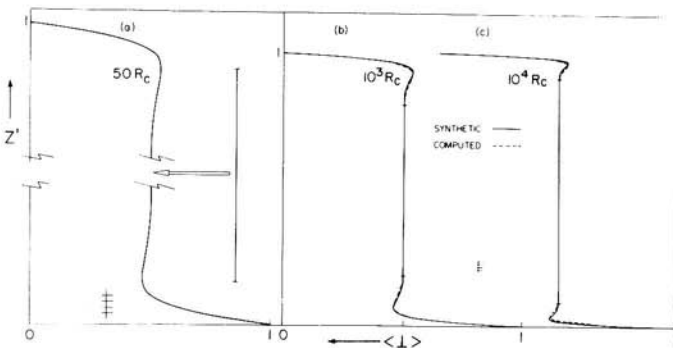
Figure 6. Construction of synthetic temperature profiles. (a) An isothermal segment of length d(f-1) is spliced into the centre of a reference profile at R_B = 50R_c . The resulting profile corresponds to that for R_B = 50f^3R_c . Examples of synthetic profiles (—), rescaled to a dimensionless height of 1, are compared with computed model profiles (---) for (b) R_B = 10^3R_c , i.e. f^3 = 20 , and (c) R_B = 10^4R_c , i.e. f^3 = 200 .
