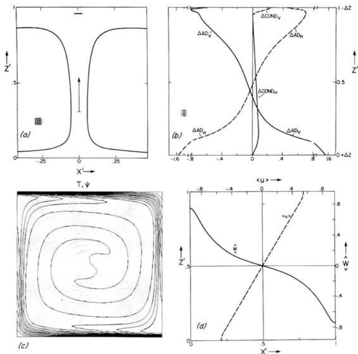
Figure 14. Characteristics of the rising plume when R_B = 10^3 R_C . (a) Shape of plume as defined by the isotherm (T_d + \Delta T/2) , that is the mean temperature contour. Direction of flow is upwards. Depth of the stagnation point thermal boundary layer is indicated by the horizontal bar above the arrow on the plume axis. Steady solution obtained on a 96 \times 96 finite-difference grid. (b) Contributions of the dimensionless flux components to the local energy balance plotted as a function of vertical distance along the centreplane of the rising plume. ( \Delta z is the vertical grid spacing. Notation as in Fig. 9.) (c) Superimposed isotherms (heavy solid curves) and streamlines (light dotted curves). (d) Horizontal variation of mean dimensionless vertical velocity \hat{W} (solid line) and vertical variation of mean dimensionless horizontal velocity \langle u \rangle (dashed line). ( \hat{W} represents the vertical average of a quantity.)
