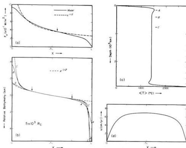
Figure 12. Model predictions for R_B = 5 \times 10^3 R_C dimensionalized using the physical parameters listed in Table 1. (a) Variation of surface heat flux across the upper surface of the convection cell (—) compared to a reference curve proportional to x^{-1/2} (---) which is constrained to have the same value as the model prediction at the point indicated by the small arrow. L is the horizontal dimension of the cell. (b) Bathymetric variation across the top of the convection cell, measured in km relative to the mid-point L/2 . The three curves labelled A, B and C result from equation (32) when compensation is assumed to occur at the depths indicated in (c) as A, B, C respectively. The dashed curve varies linearly with x^{1/2} and is constrained to fit curve B at the points indicated by the small arrows. (c) Mean vertical temperature profile. Depths A, B and C indicate values of z_1 (equation 32) used in (b). (d) Variation of horizontal surface velocity across the top of the convection cell.
