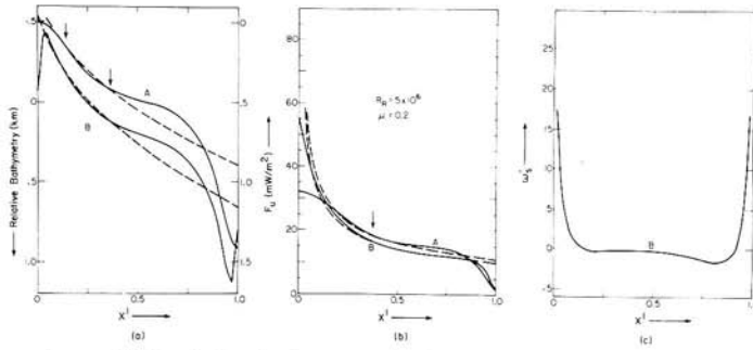
Figure 24. Comparison of (a) relative bathymetry, D_2(x) , and (b) surface heat flux, F_u , as computed from the model solutions with free-slip upper boundary conditions (curves labelled A) and constant velocity upper boundary condition (curves labelled B). D_2 and F_u have been dimensionalized using the parameter values listed in Table 1. In (a) the left ordinate scale refers to curve B while the right scale refers to curve A. (c) Variation of dimensionless vorticity at the upper surface, \omega'_s , in the case of the constant velocity upper surface.
